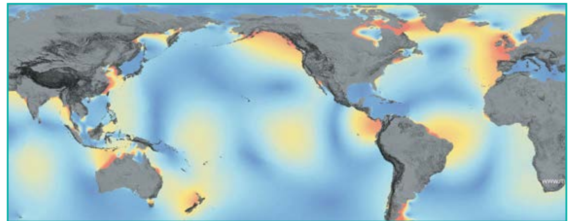
Figure 2: World Distribution Map of Tidal Range
